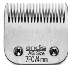
Item #64121 Size 7 Finish Cut Leaves hair 1/8" - 3.2mm
